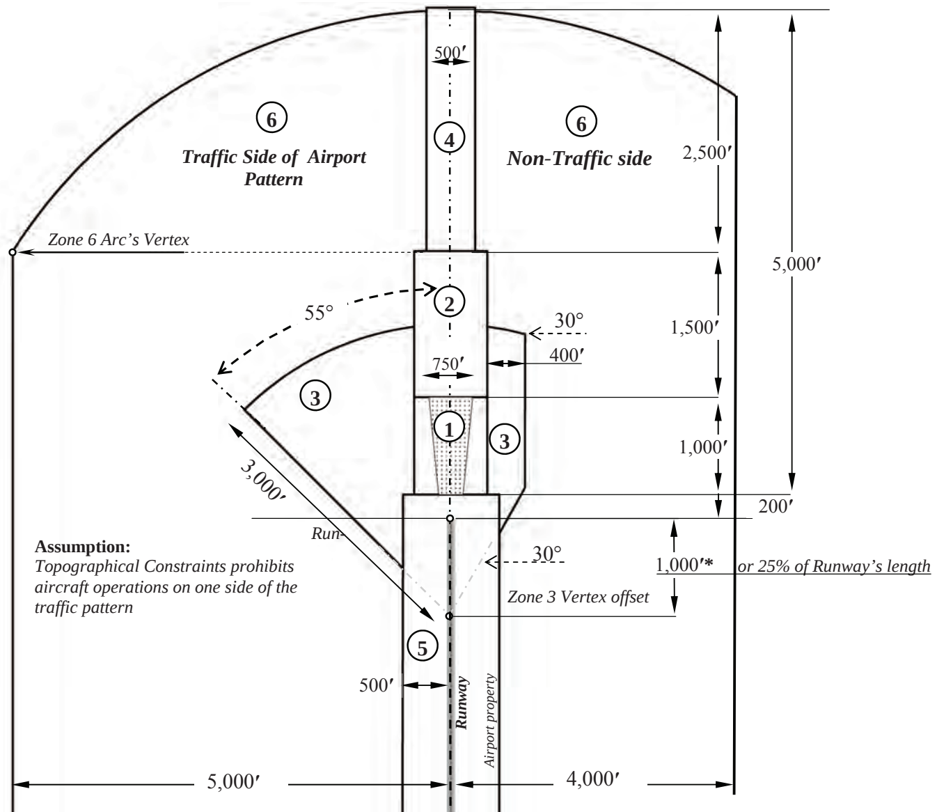
Airport Compatibility Zones
