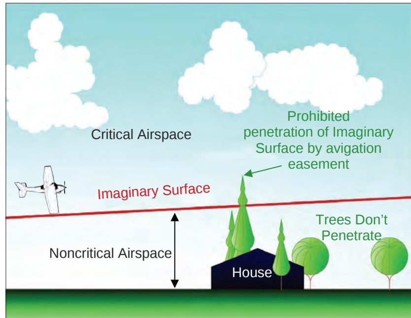
Avigation Easements May Be Used To Protect Critical Airspace
